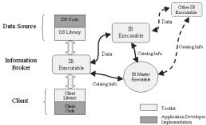
Figure 1: An Instantiation of a DBIS
